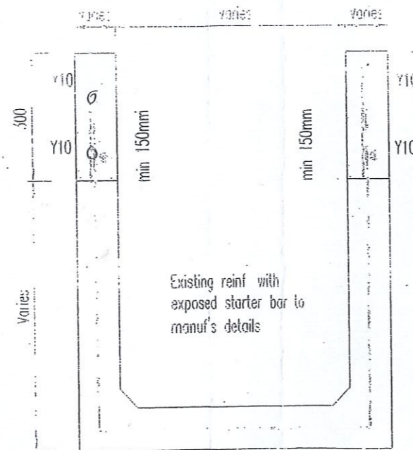
PLAN OF CAPPING BEAM
