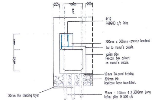
SECTION C-C
