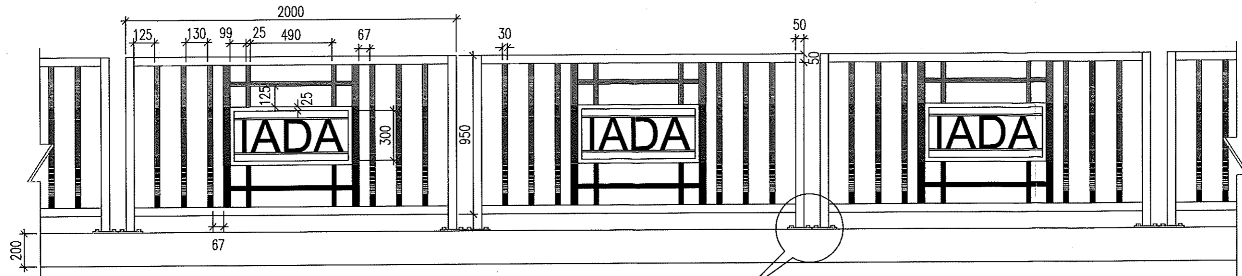
FRONT ELEVATION
